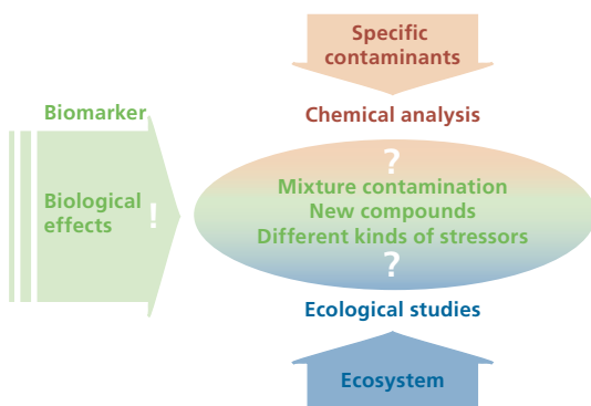
Figure 2.36 Diagram showing the integrating role of biological effects within the impact assessment of environmental pollution.
