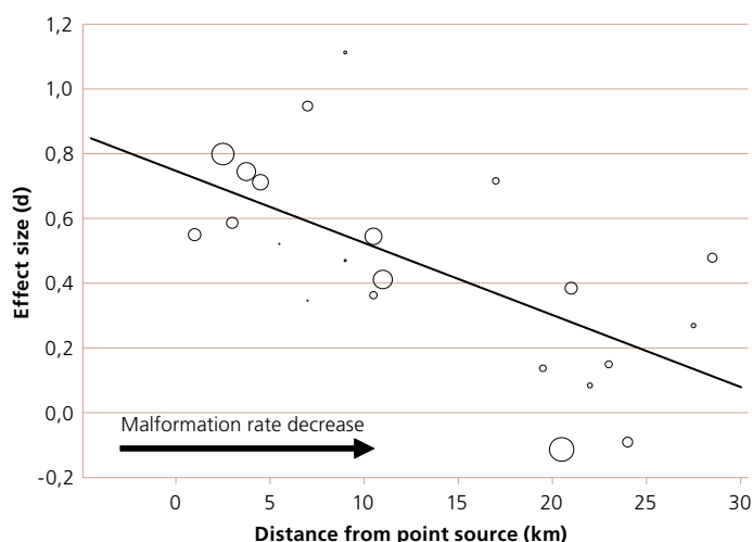
Figure 2.44 The proportion of malformed embryos in the amphipod Monoporeia affinis increases with decreasing distance from the point source, suggesting that there is a strong relationship between the emission sources studied and the malformation rate. The analysis includes results from a total of 24 sampling stations from six regional studies at polluted recipient areas. Results have been transformed into "effect sizes" in order to make the studies comparable (mean-centred and scaled with 1/SD).
