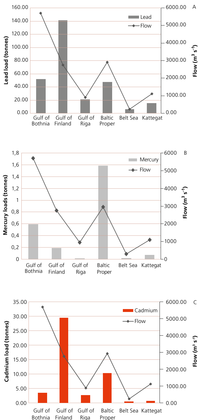
Figure 3.4 Total waterborne inputs of A) lead, B) mercury and C) cadmium to the Baltic Sea sub-basins in 2006 (Knuuttila 2009). The flow ( \text{m}^3 \text{s}^{-1} ) indicates the average annual riverine inflow entering each sub-basin. The mercury load from River Vistula has been removed due to unreliable monitoring data.
