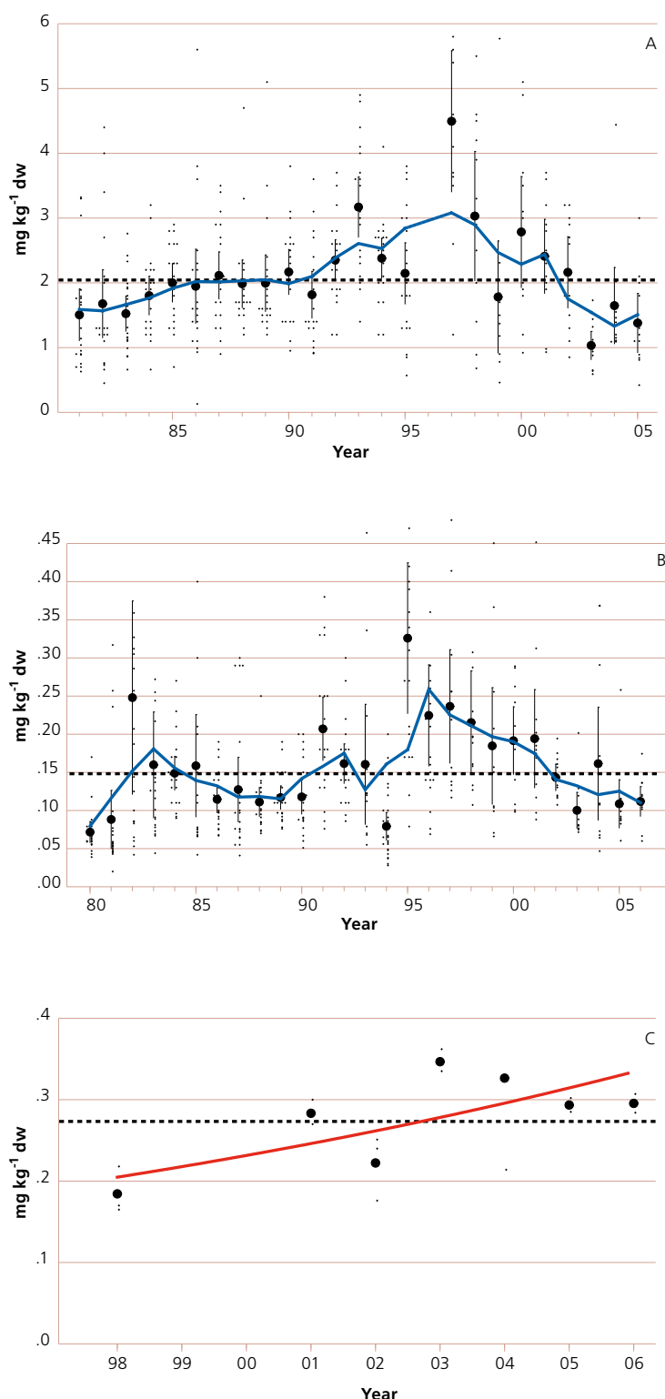
Figure 2.14 Temporal trends of concentrations (in mg kg -1 dw) of (A) cadmium and (B) mercury in fish from Landsort (Northern Baltic Proper) and (C) mercury in blue mussels from the southern part of the Sound. The horizontal dashed line shows the overall geometric mean of the data and the solid line indicates the smoothed average of the measurements (blue) or the trend (red).
