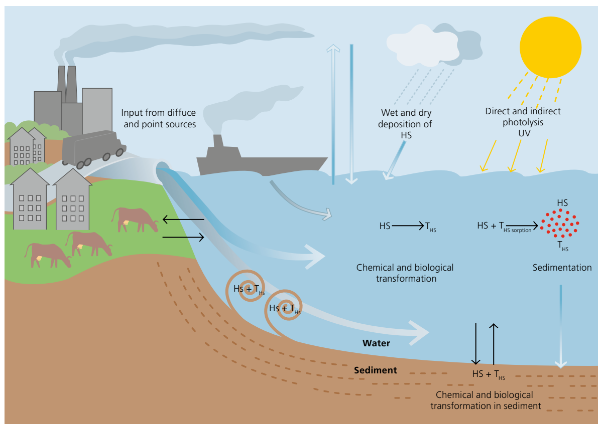
Figure 1.2 Conceptual model of the sources of pollution inputs to the Baltic Sea marine environment and the fate of hazardous substances (HSs) and their transformation products ( T_{HS} ) (based on Dahllöf & Andersen (2009)).
