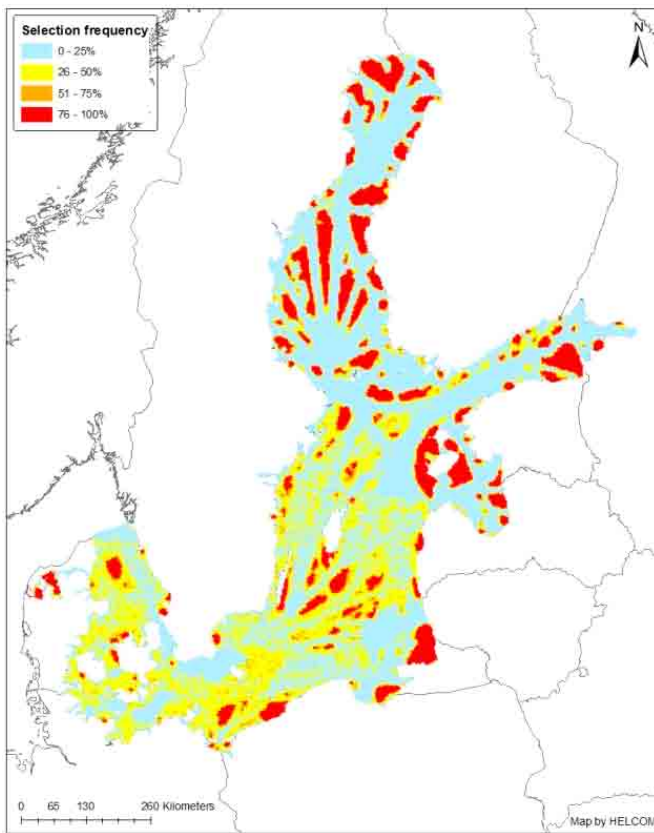
Figure 8. Selection frequency of different areas with a) lower; and b) higher conservation targets with minimum 30% sub-regional coverage. Existing MPAs were not included. For conservation targets see Tables 49 and 50 in the report.
