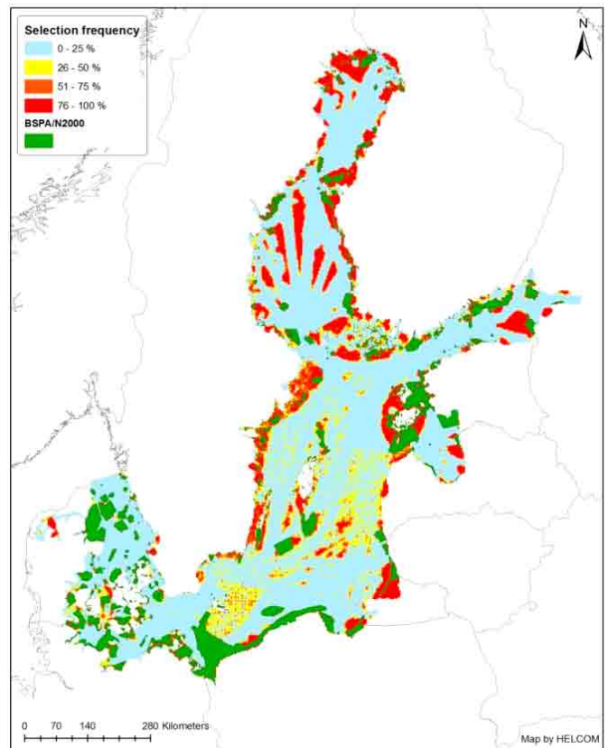
Figure 4. Selection frequency of different areas with a) lower; and b) higher conservation targets with minimum 30% sub-regional coverage with existing MPAs included. For conservation targets see Tables 49 and 50 in the report.
