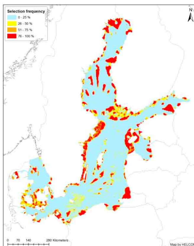
Figure 7. Selection frequency of different areas with a) lower; and b) higher conservation targets with minimum 20% sub-regional coverage. Existing MPAs were not included. For conservation targets see Tables 49 and 50 in the report.
