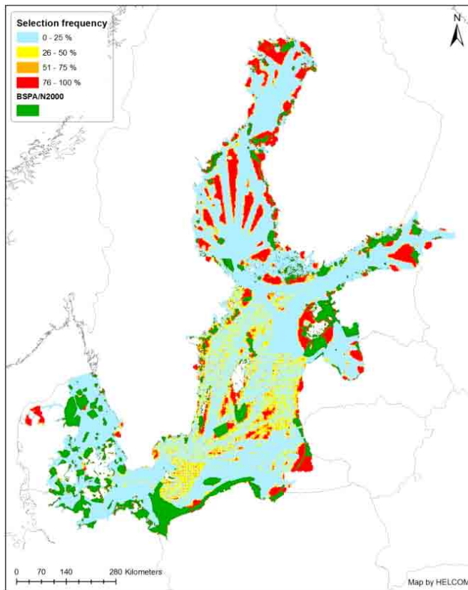
Figure 4. Selection frequency of different areas with a) lower; and b) higher conservation targets with minimum 30% sub-regional coverage with existing MPAs included. For conservation targets see Tables 49 and 50 in the report.
