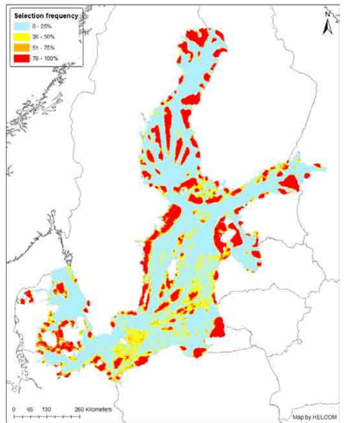
Figure 8. Selection frequency of different areas with a) lower; and b) higher conservation targets with minimum 30% sub-regional coverage. Existing MPAs were not included. For conservation targets see Tables 49 and 50 in the report.
