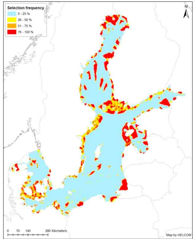
Figure 6. Selection frequency of different areas with a) lower; and b) higher conservation targets with minimum 12% sub-regional coverage. Existing MPAs were not included. For conservation targets see Tables 49 and 50 in the report.
