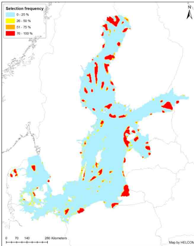
Figure 6. Selection frequency of different areas with a) lower; and b) higher conservation targets with minimum 12% sub-regional coverage. Existing MPAs were not included. For conservation targets see Tables 49 and 50 in the report.
