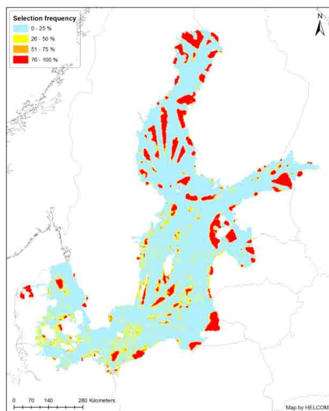
Figure 7. Selection frequency of different areas with a) lower; and b) higher conservation targets with minimum 20% sub-regional coverage. Existing MPAs were not included. For conservation targets see Tables 49 and 50 in the report.
