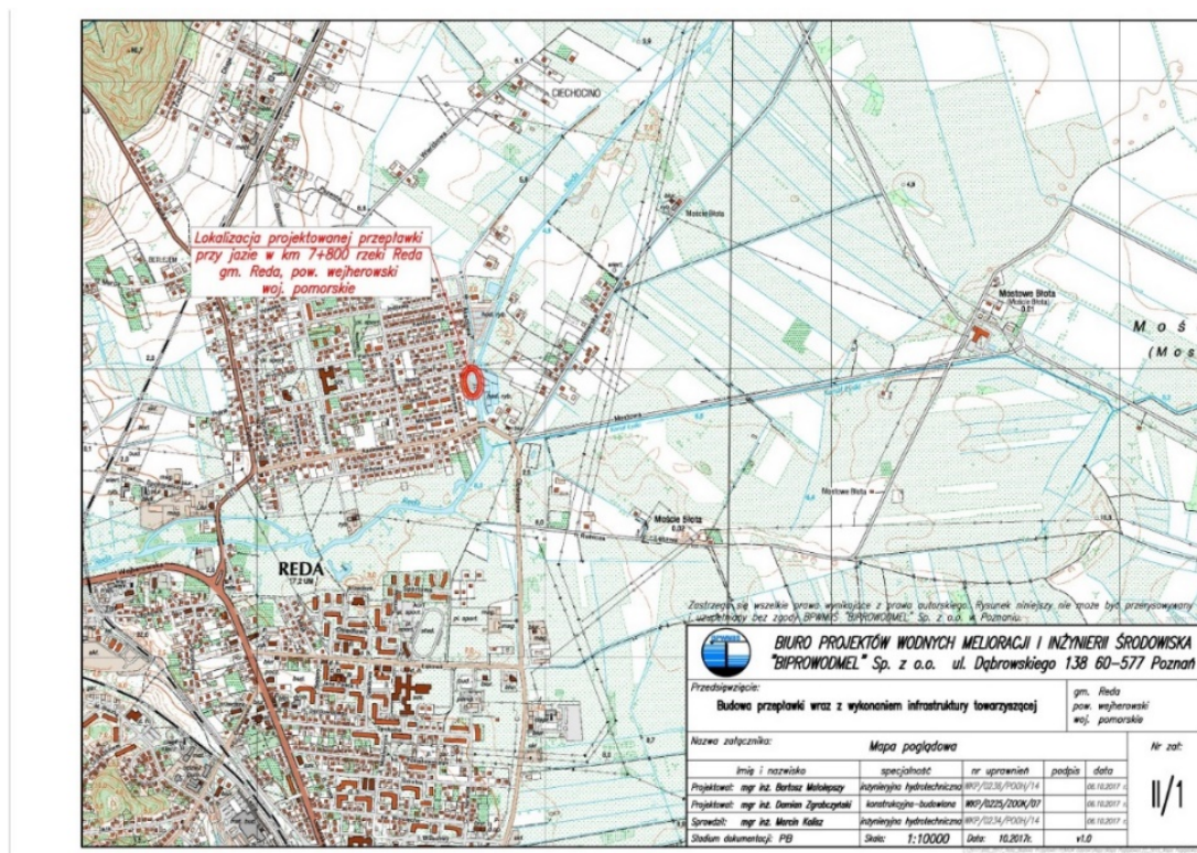
Figure 35. Detailed location of the planned fish pass in Reda. Credits: National Water Holding "Polish Waters".
