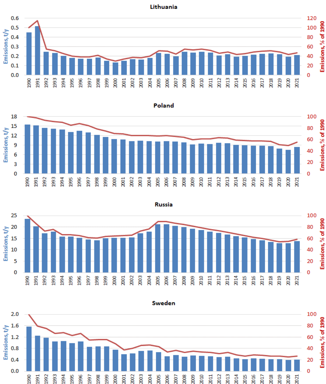
Figure 3 (continued). Mercury emissions of the HELCOM Contracting Parties (CP) to the atmosphere for the period 1990-2021 in \text{t y}^{-1} (blue bars) and in % of 1990 (red line). The emission data of the CP refer to the total area of the CPs except for Russia, where emissions from the territory of Russia within the EMEP domain is used.
