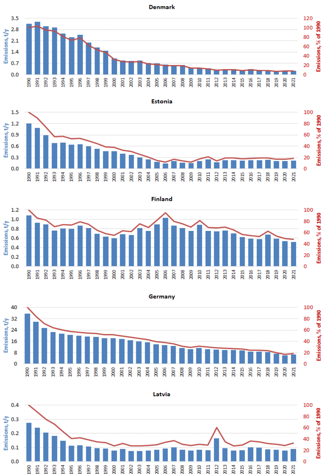
Figure 3. Mercury emissions of the HELCOM Contracting Parties (CP) to the atmosphere for the period 1990-2021 in \text{t y}^{-1} (blue bars) and in % of 1990 (red line). The emission data of the CP refer to the total area of the CP except for Russia, where emissions from the territory of Russia within the EMEP domain is used.
