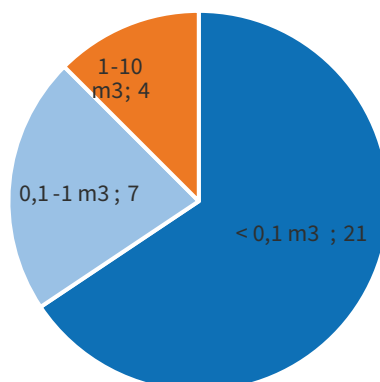
Figure 7. Oil discharges detected in the Baltic Sea during aerial surveillance in 2023 according to estimated volume (m3) of the spill.
