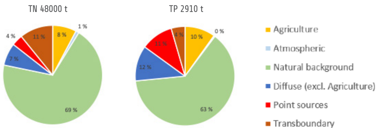
Figure 38. Total nitrogen (TN) and total phosphorus (TP) loads exported by the Neva River in 2021 divided into load sources.
